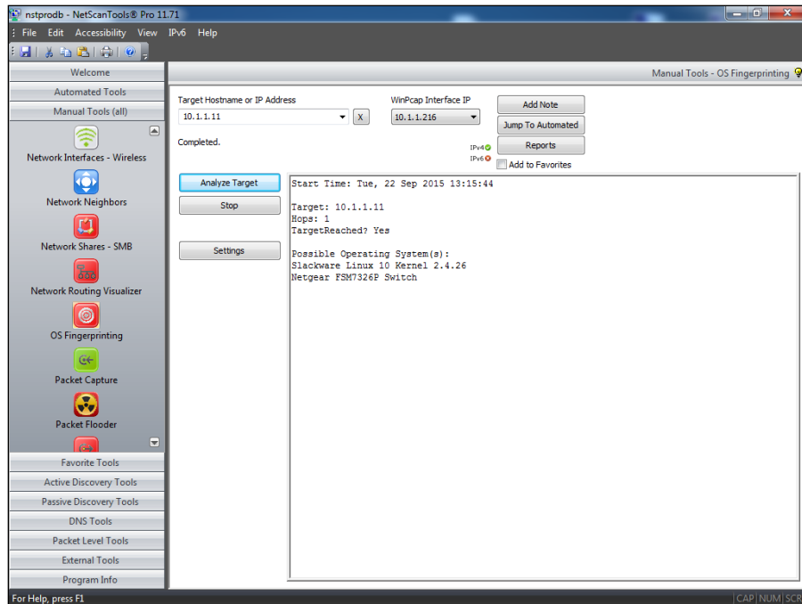
Figure 13-5: Using NetScan- Tools Pro to determine that Slack- ware Linux is likely running.
